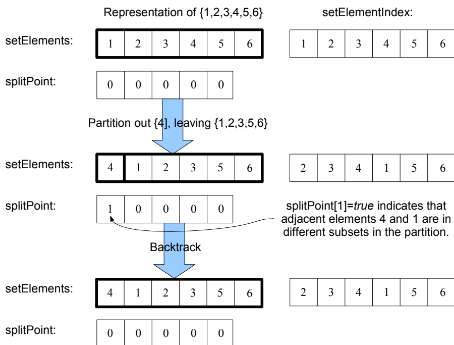
FIGURE 4.3. Illustration of partitioning element 4 from the set \{1,2,3,4,5,6\}
